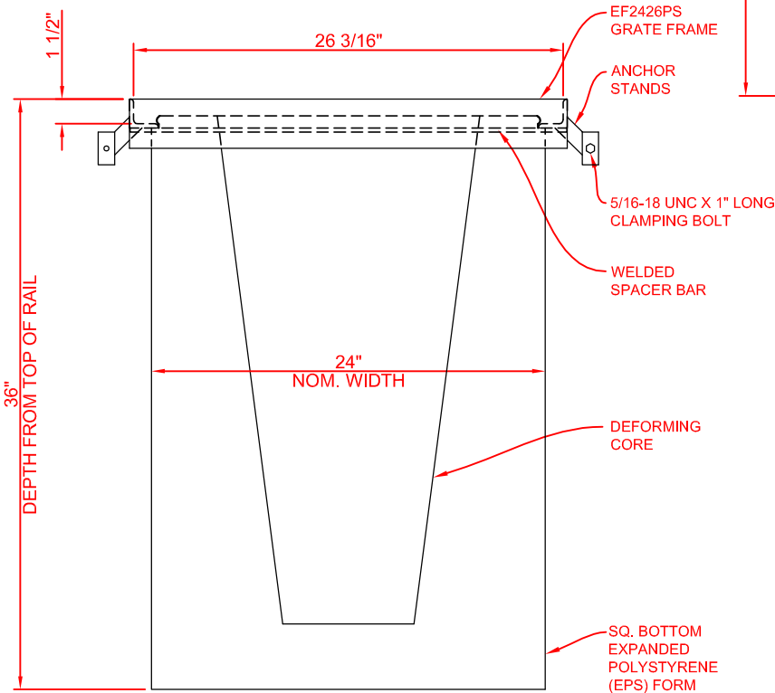
END VIEW
