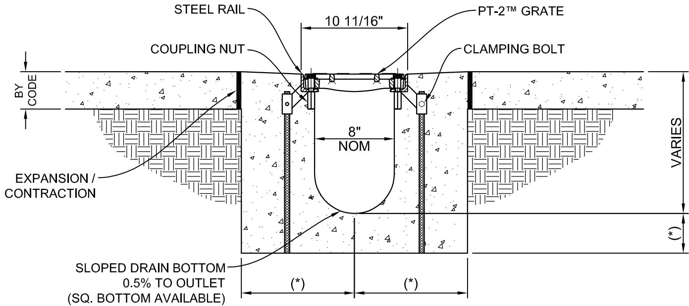
SECTION DO NOT SCALE
