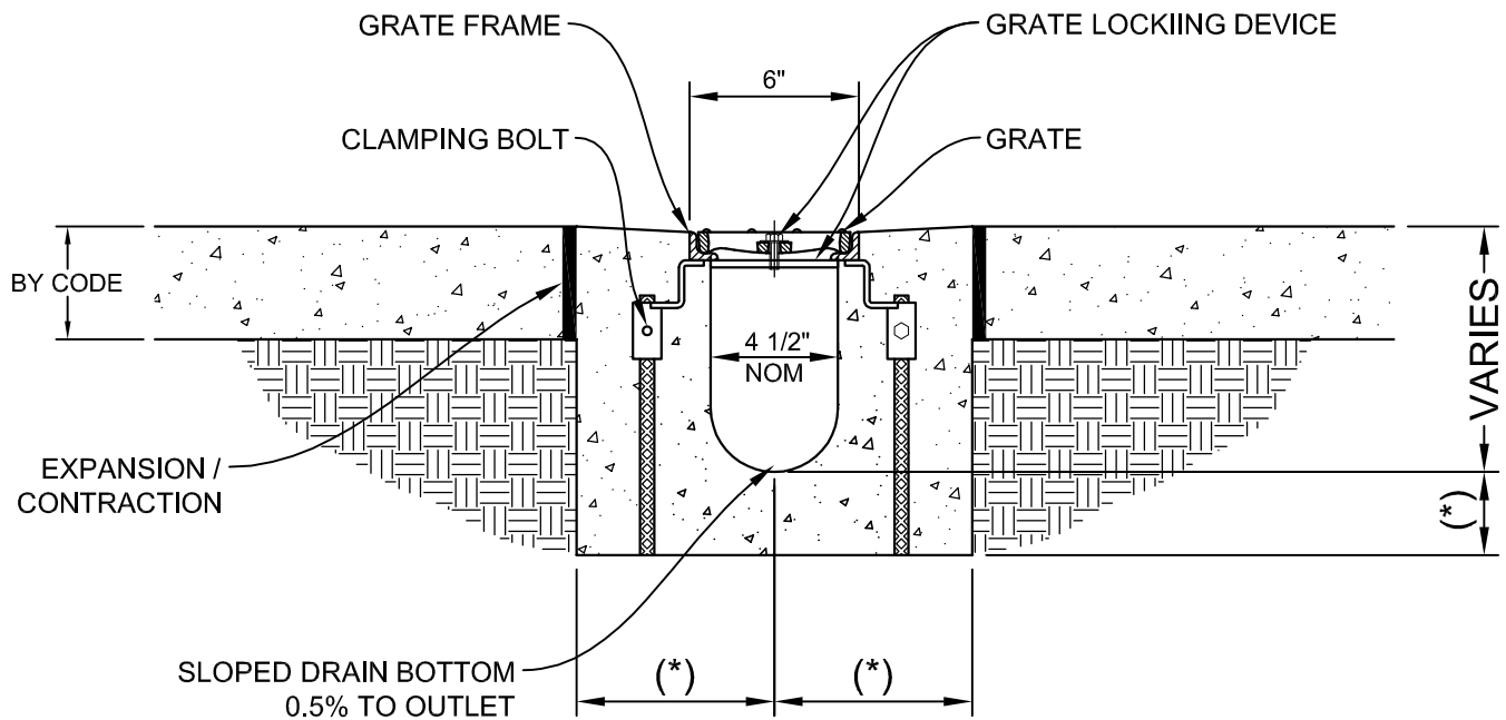
SECTION DO NOT SCALE
